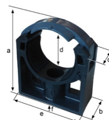
FIXING CLAMP D50 EX
